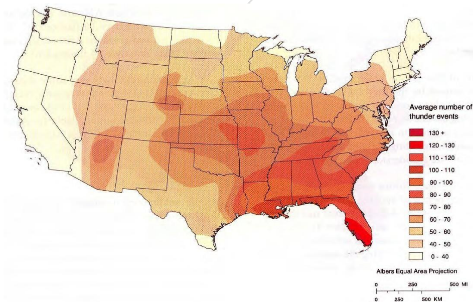
Figure 3-1: Annual Average Number of Thunder Events
